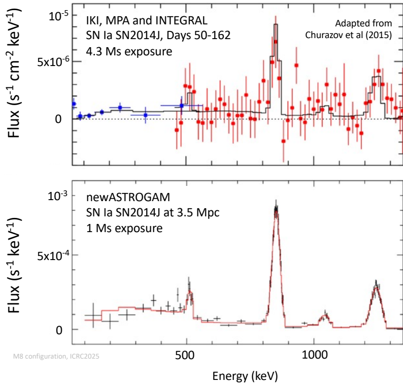
Figure 2: Improvement over INTEGRAL (top, [13]) for a type-Ia SN. Lines from the ^{56}Ni decay chain will clearly be resolved (bottom), yielding the radioactive and total ejecta masses, a characteristic of the progenitors.
